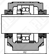
TYPE TS LABYRINTH SEALS
