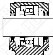
TYPE TC FELT SEALS
