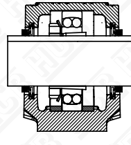
TYPE TA V-RING SEALS
